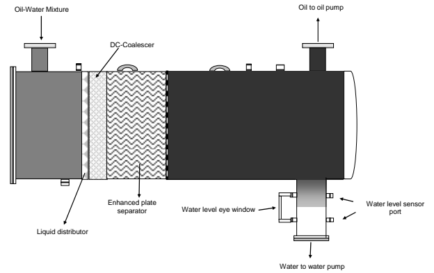
Figure 3 Schematic of internal components in oil-water separator
