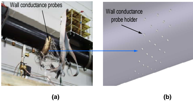
Figure 5 Wall conductance probes (a): wall conductance probes on the test section (b): 5 rows of staggered configuration of probe holders
