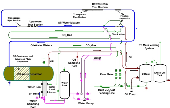
Figure 2. Schematic of 4-inch I.D. fully Inclined multiphase flow loop
