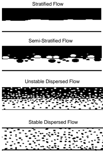
Figure 1. Flow patterns in oil-water horizontal flows
